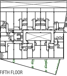
FIFTH FLOOR
